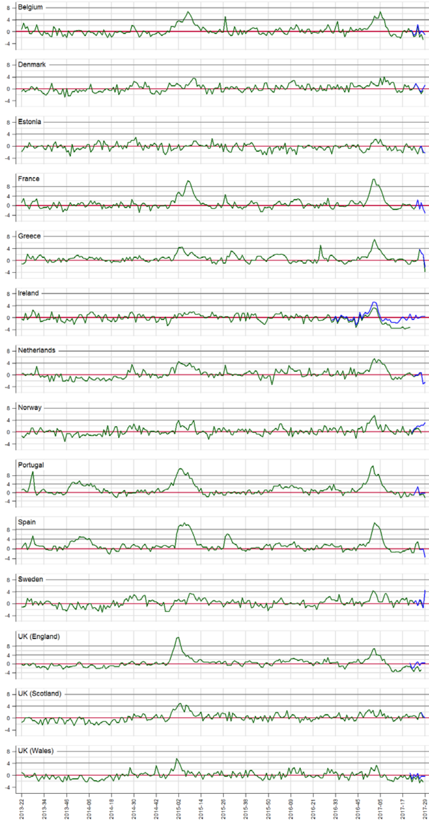
Weekly z-score, age group Total by country EuroMOMO: week 29, 2017
